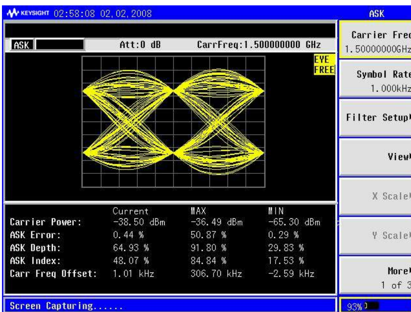
The Eye Diagram of ASK also shows the metrics with detailed parameters.
